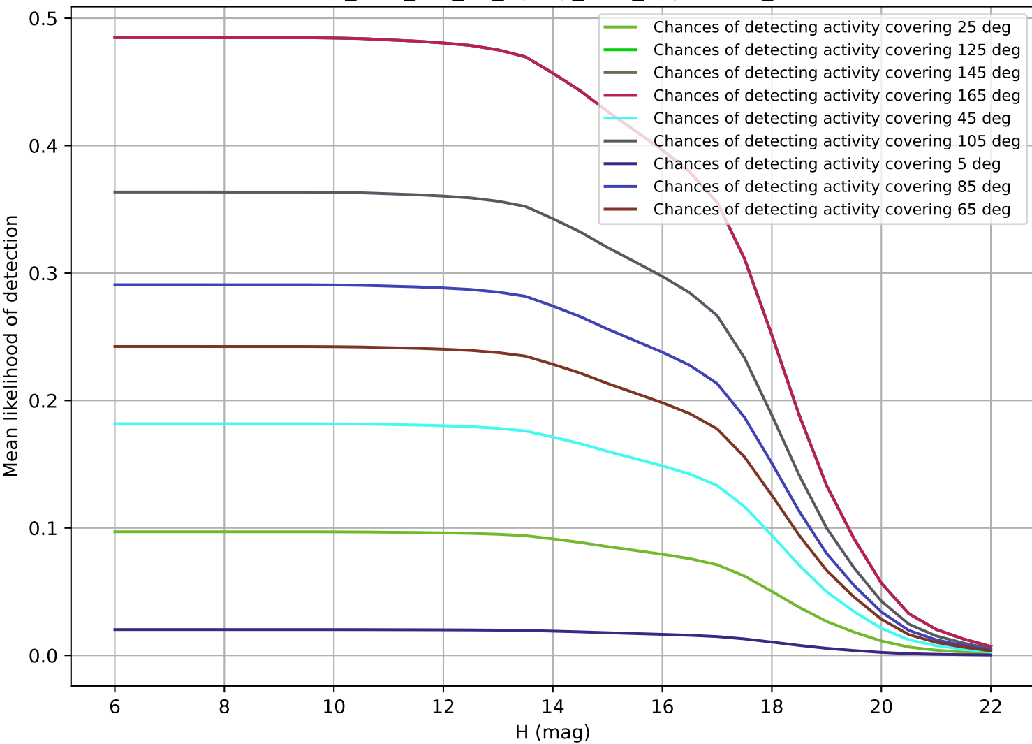
too_elab_r32_d3_ugrizy_v3.4_10yrs OCC_r5
