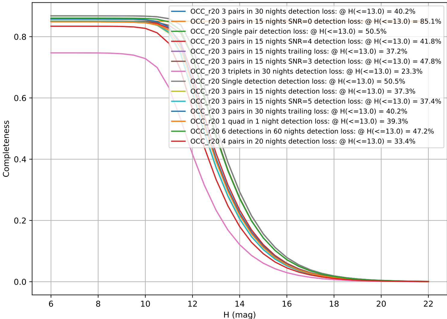
too_elab_r32_d3_ugrizy_v3.4_10yrs: CumulativeCompleteness
