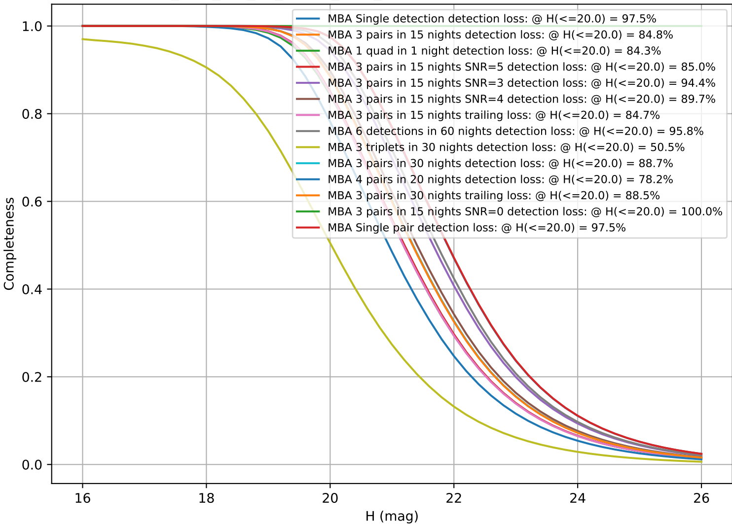
too_elab_r32_d3_ugrizy_v3.4_10yrs: CumulativeCompleteness
