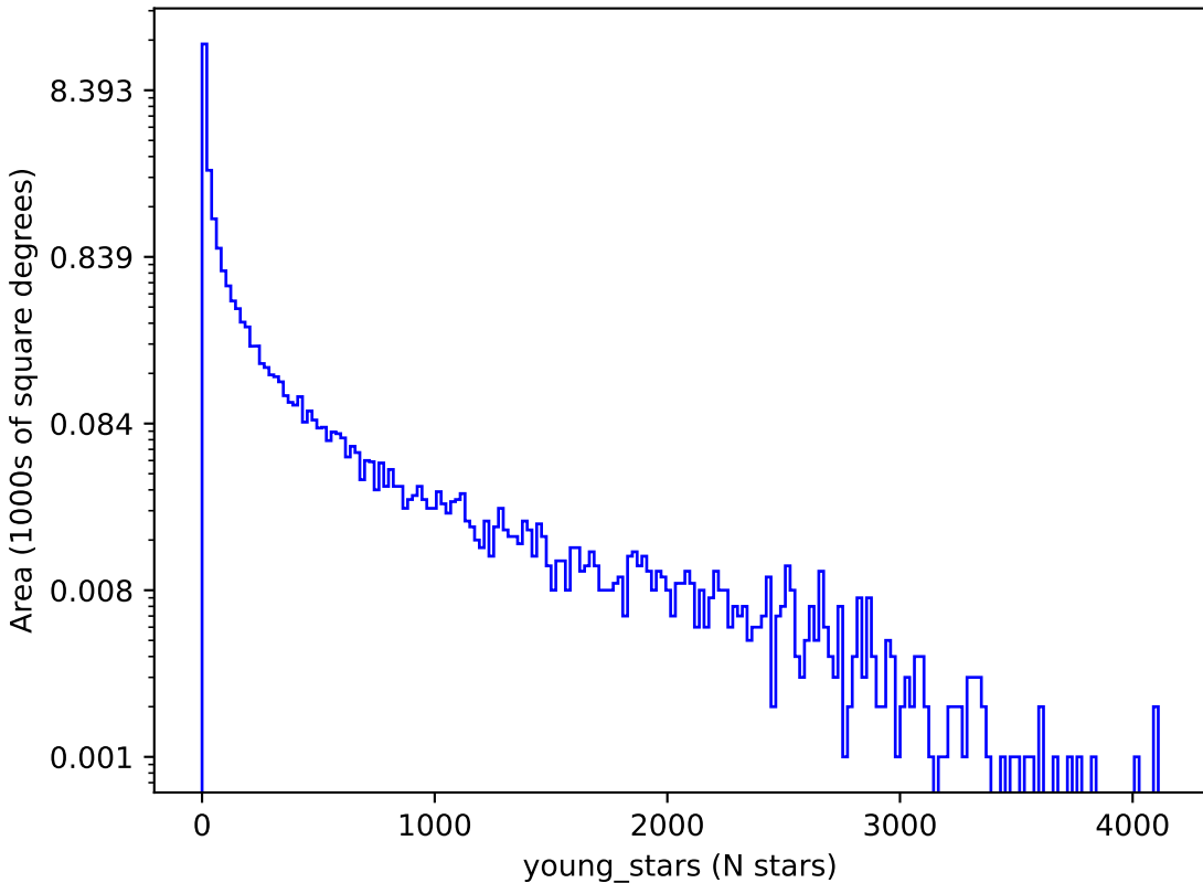
too_elab_r32_d3_ugrizy_v3.4_10yrs : young_stars
