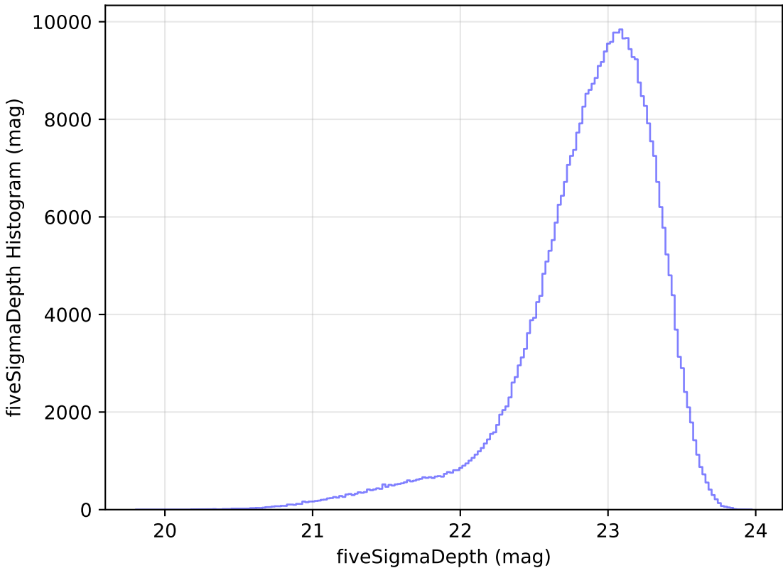
too_elab_r32_d3_ugrizy_v3.4_10yrs z: fiveSigmaDepth Histogram
