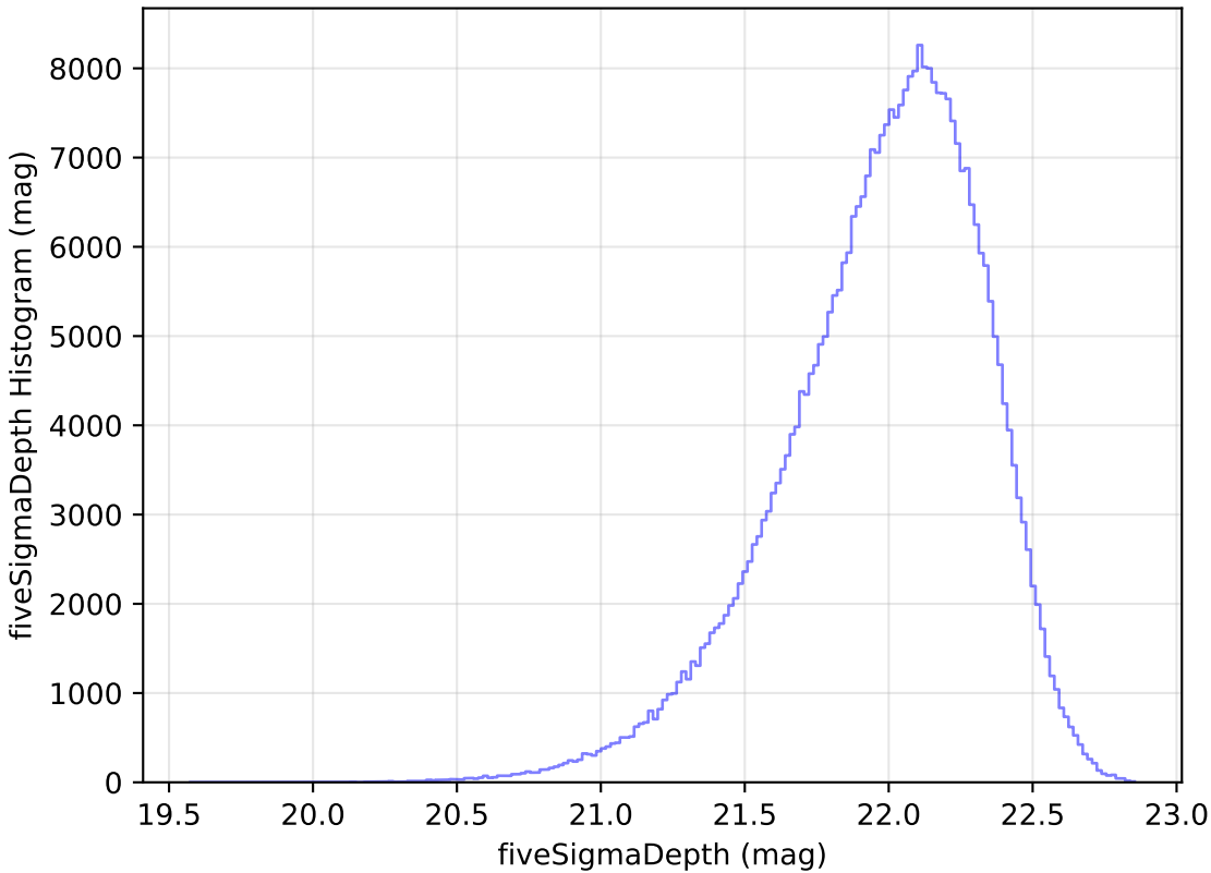
too_elab_r32_d3_ugrizy_v3.4_10yrs y: fiveSigmaDepth Histogram
