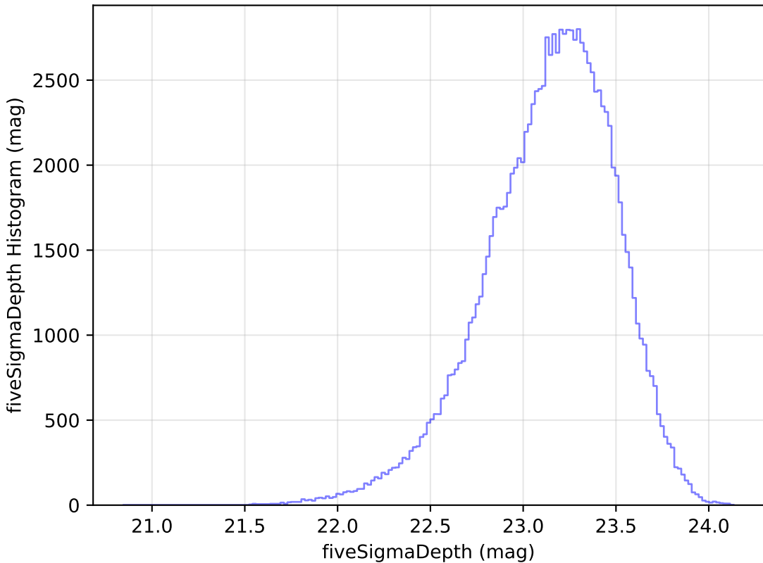
too_elab_r32_d3_ugrizy_v3.4_10yrs u: fiveSigmaDepth Histogram
