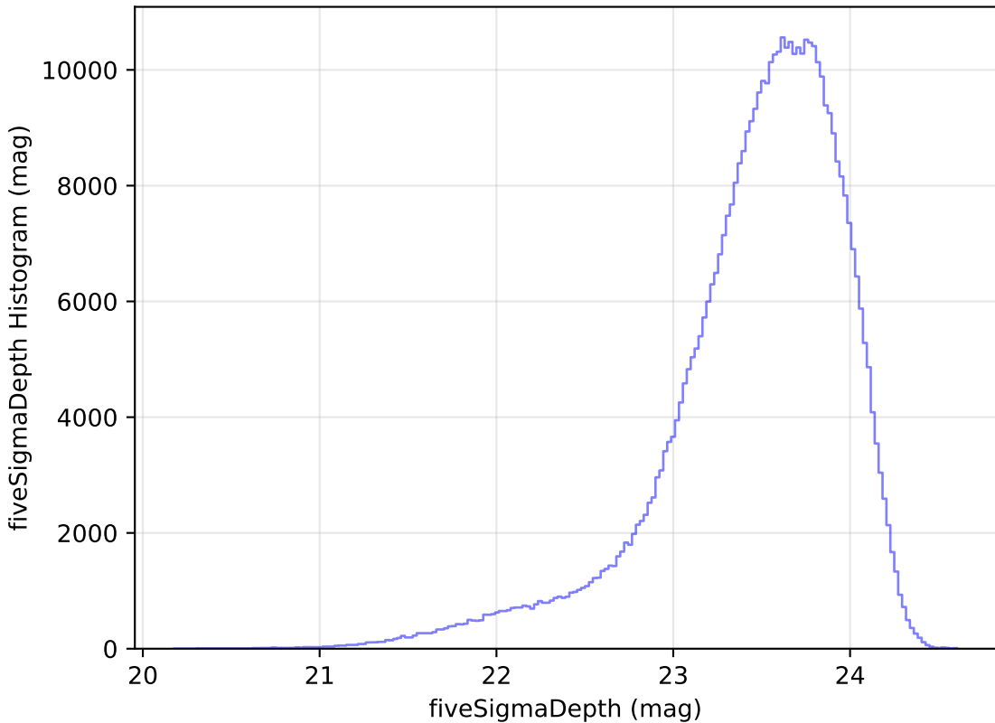
too_elab_r32_d3_ugrizy_v3.4_10yrs i: fiveSigmaDepth Histogram
