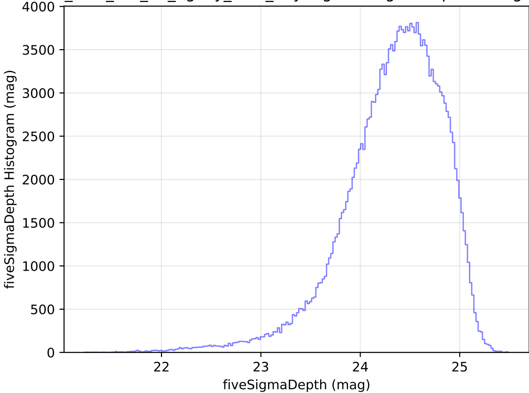
too_elab_r32_d3_ugrizy_v3.4_10yrs g: fiveSigmaDepth Histogram
