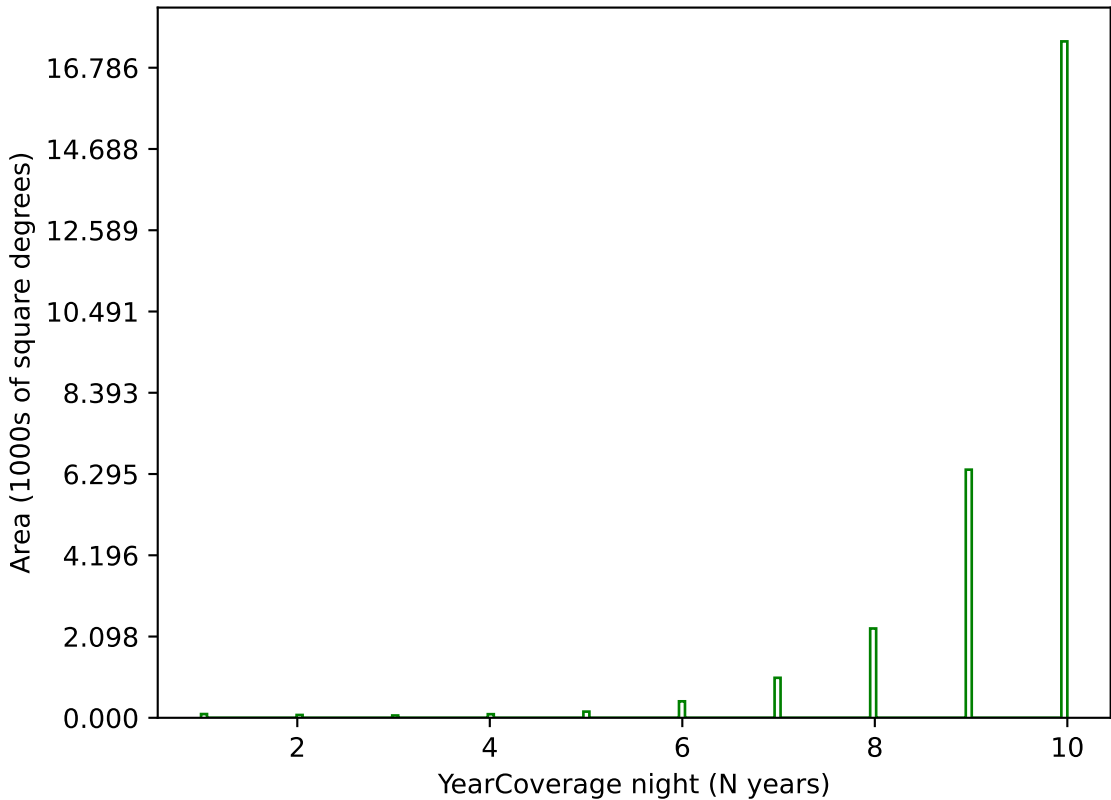
too_elab_r32_d3_uigrizy_v3.4_10yrs g band: YearCoverage night
