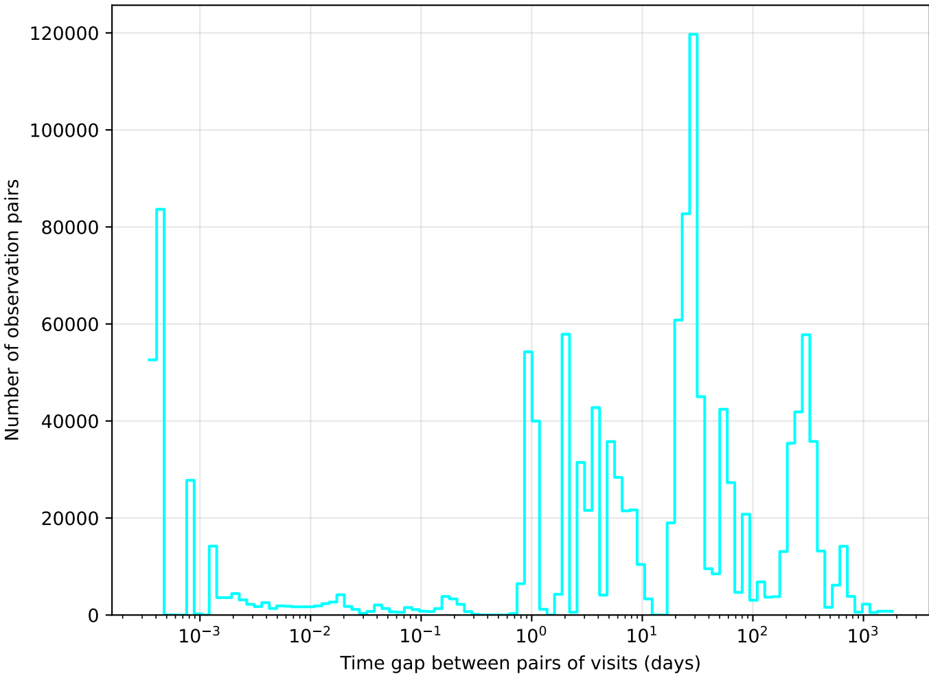
too_elab_r32_d3_ugrizy_v3.4_10yrs u band: Tgaps observationStartMJD
