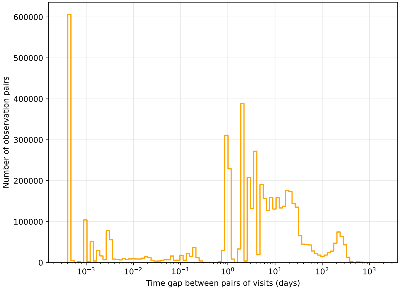
too_elab_r32_d3_ugrizy_v3.4_10yrs r band: Tgaps observationStartMJD
