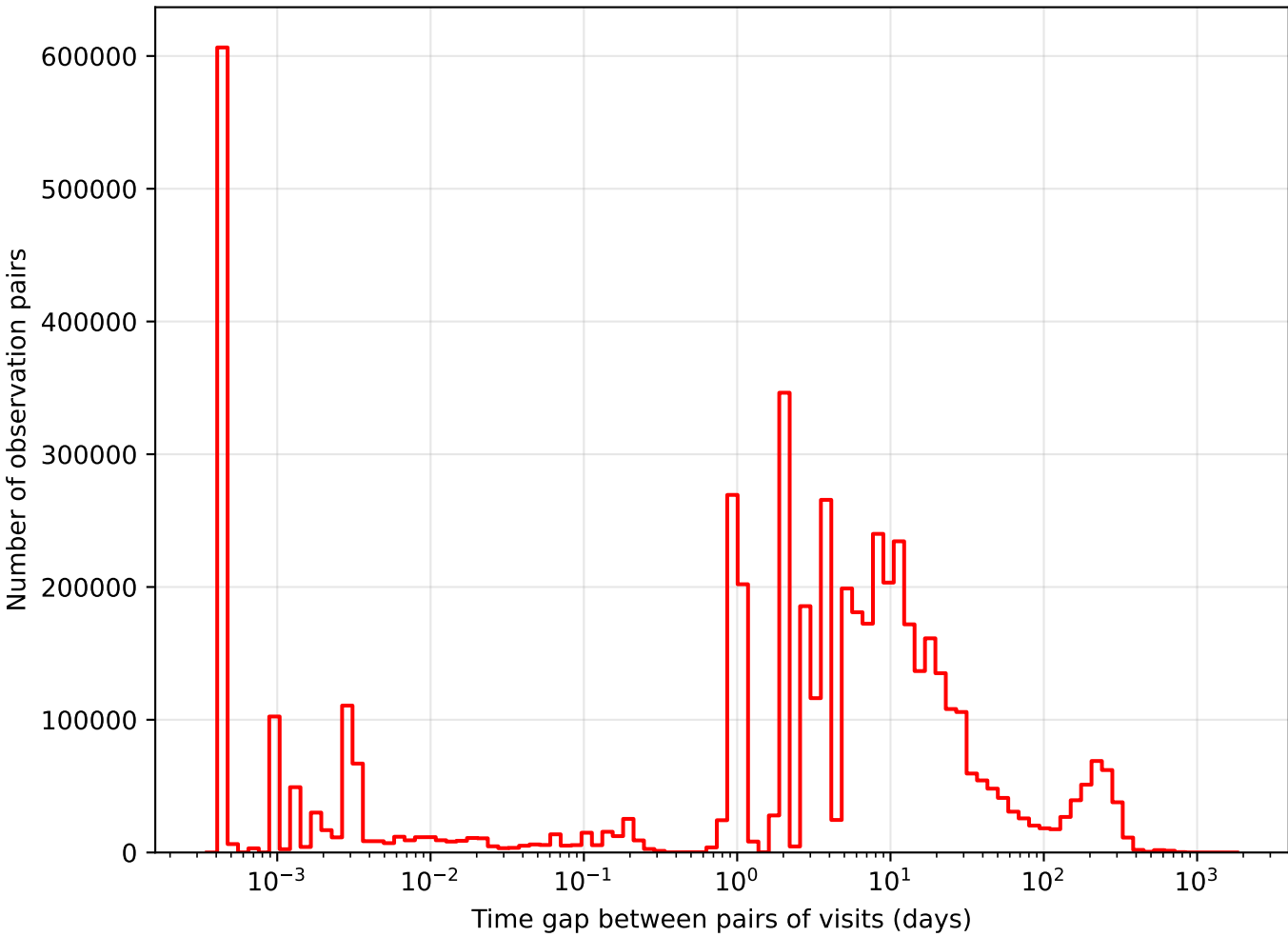
too_elab_r32_d3_ugrizy_v3.4_10yrs i band: Tgaps observationStartMJD
