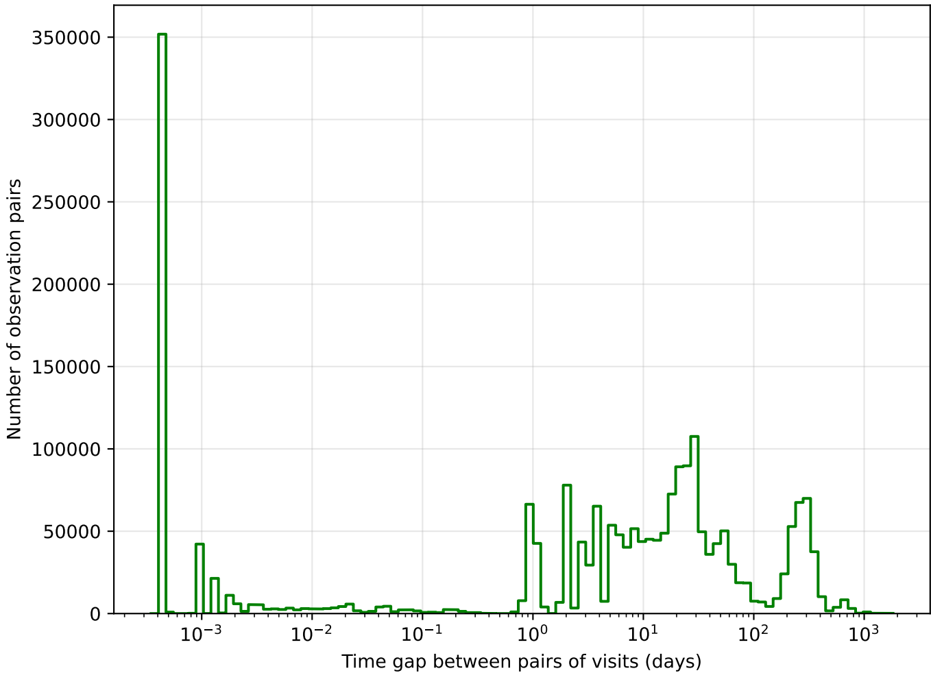
too_elab_r32_d3_ugrizy_v3.4_10yrs g band: Tgaps observationStartMJD
