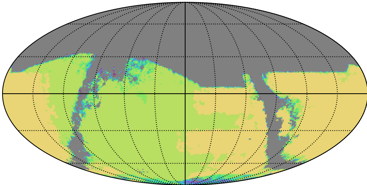
too_elab_r32_d3_ugrizy_v3.4_10yrs : TDC_campaign
