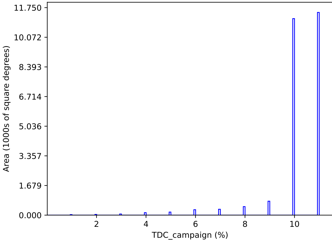
too_elab_r32_d3_ugrizy_v3.4_10yrs : TDC_campaign
