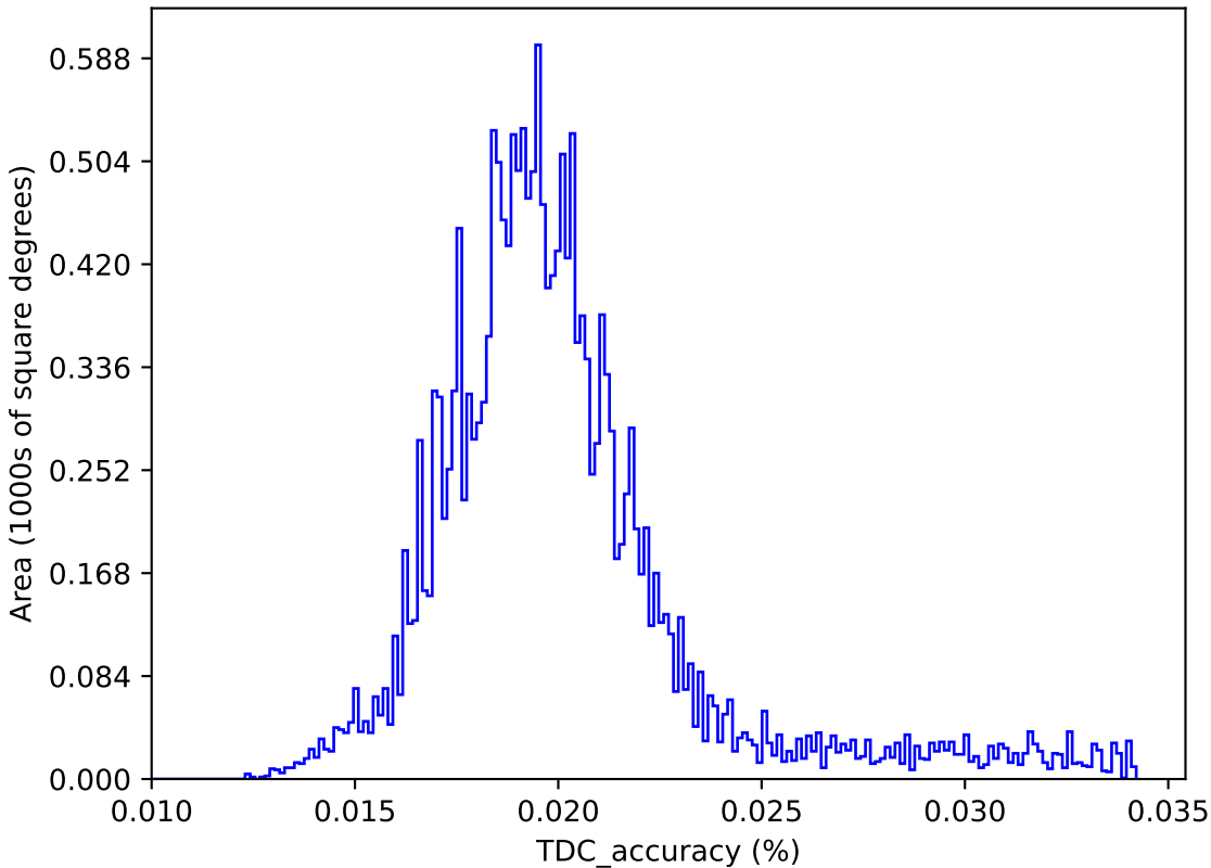
too_elab_r32_d3_ugrizy_v3.4_10yrs : TDC_accuracy
