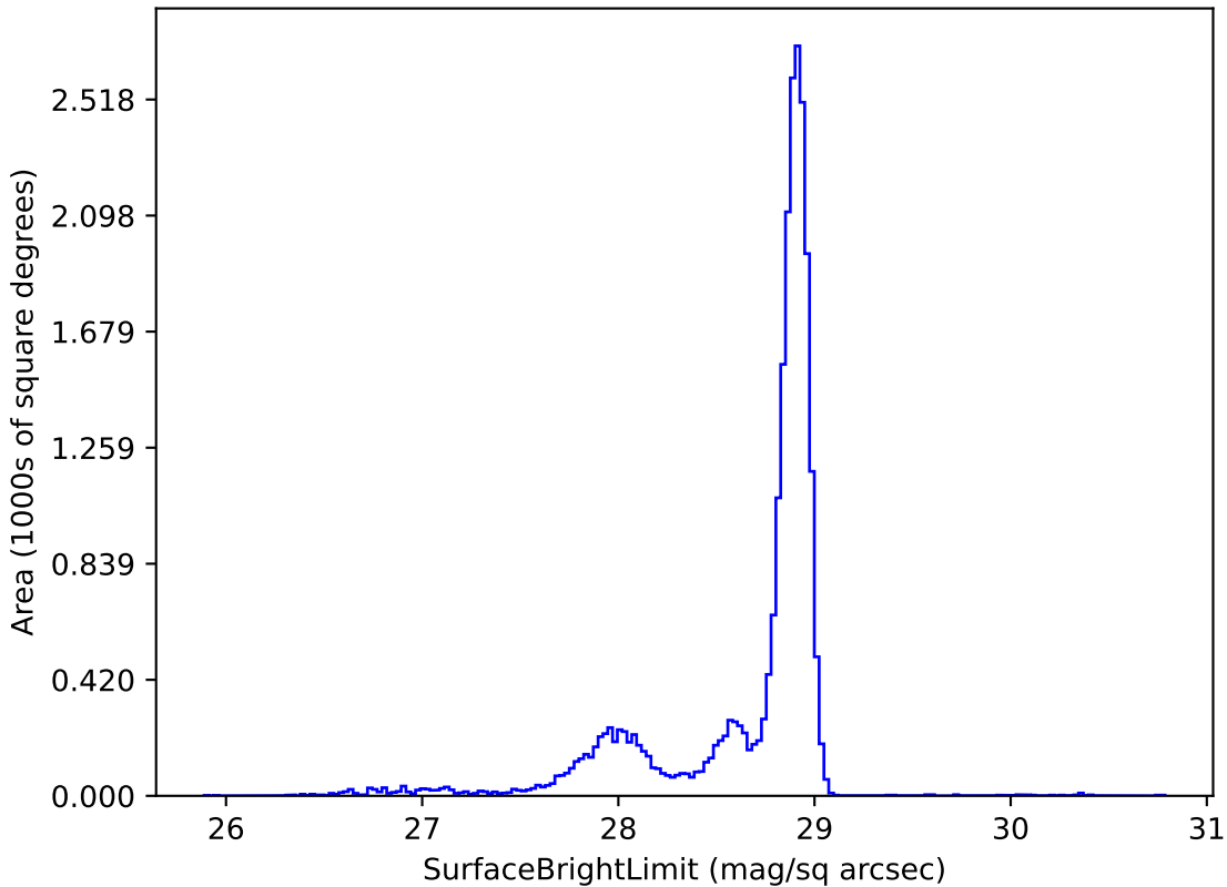
too_elab_r32_d3_ugrizy_v3.4_10yrs u: SurfaceBrightLimit
