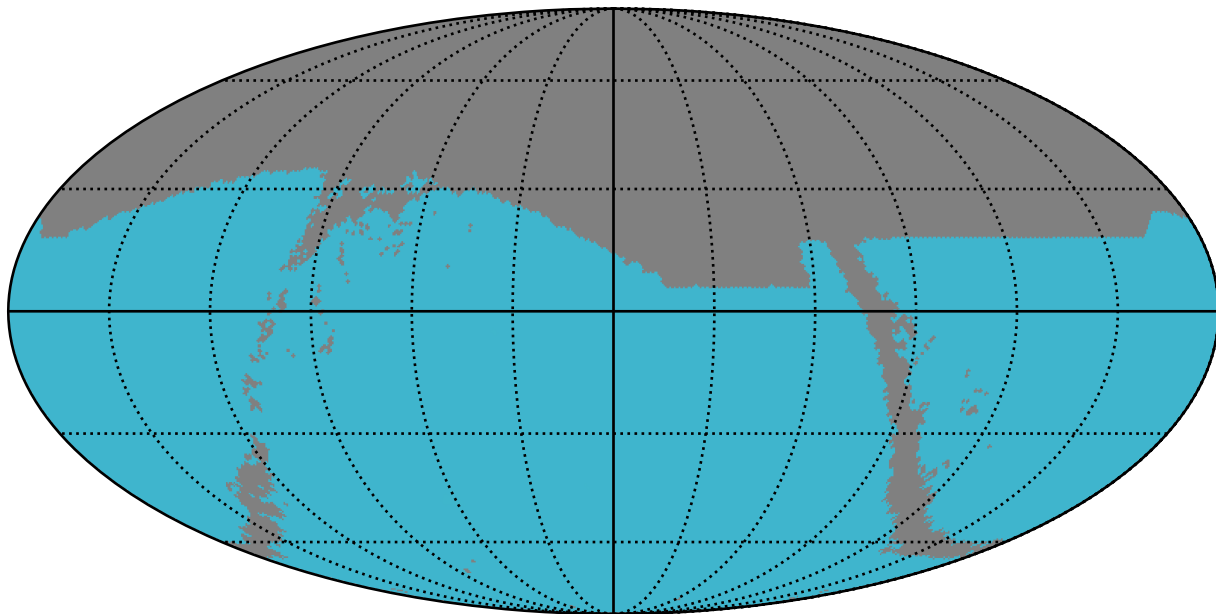
too_elab_r32_d3_ugrizy_v3.4_10yrs : SNSLMetric
