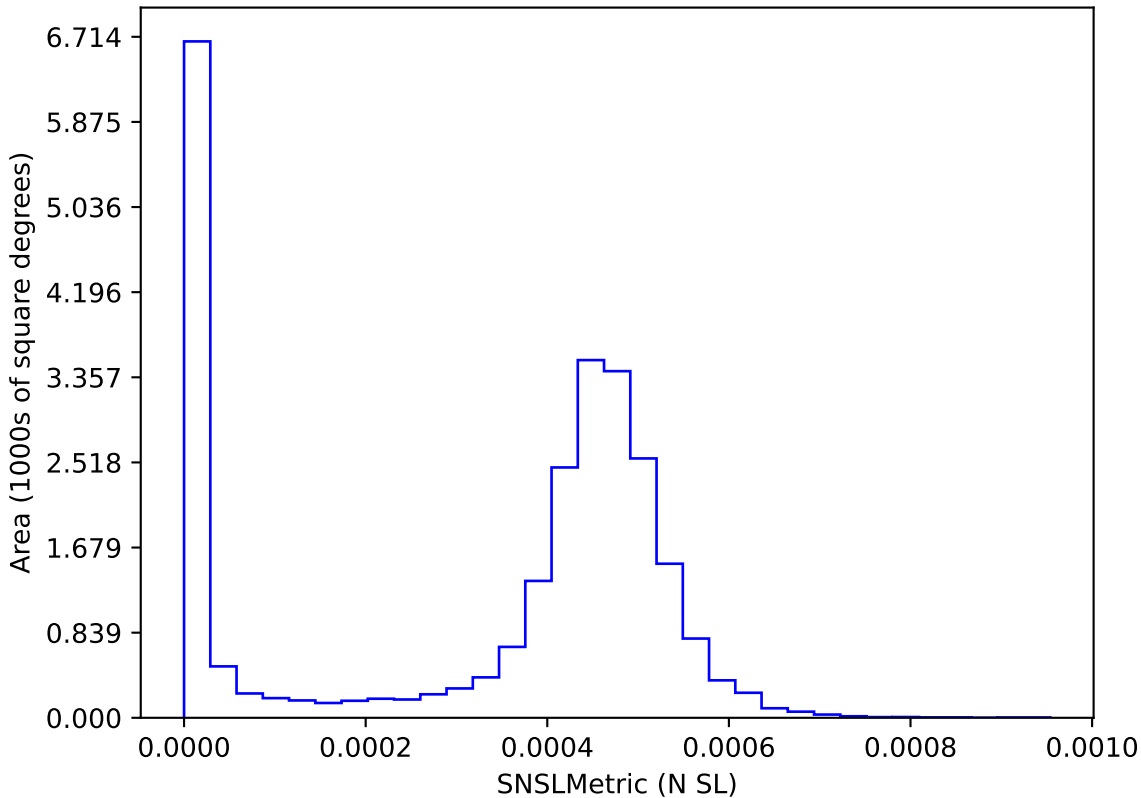
too_elab_r32_d3_ugrizy_v3.4_10yrs : SNSLMetric
