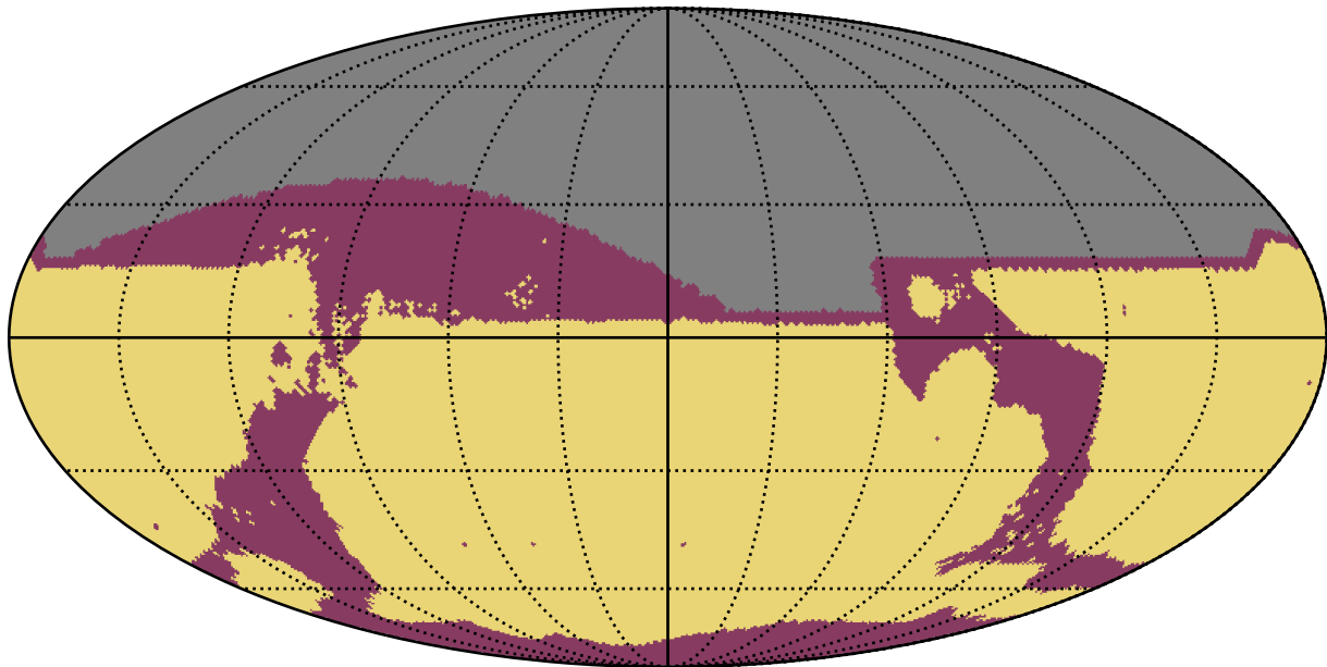
too_elab_r32_d3_ugrizy_v3.4_10yrs : RapidRevisits
