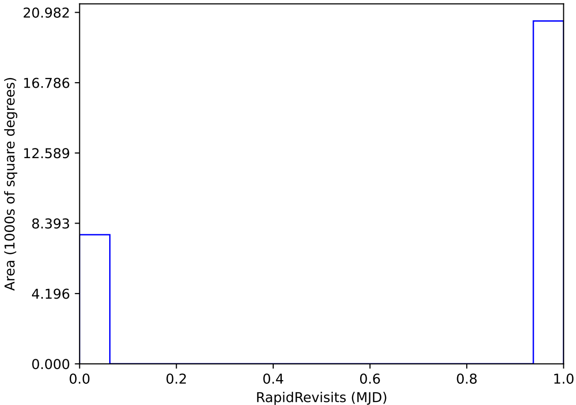
too_elab_r32_d3_ugrizy_v3.4_10yrs : RapidRevisits
