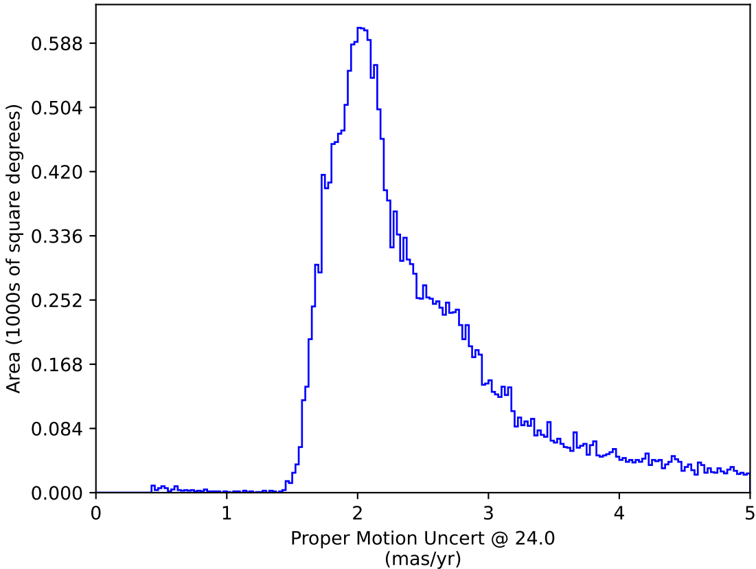
too_elab_r32_d3_ugrizy_v3.4_10yrs : Proper Motion Uncert @ 24.0
