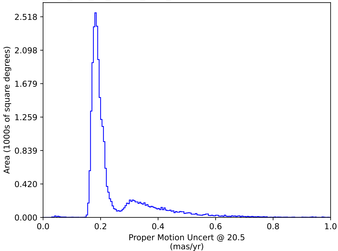
too_elab_r32_d3_ugrizy_v3.4_10yrs : Proper Motion Uncert @ 20.5
