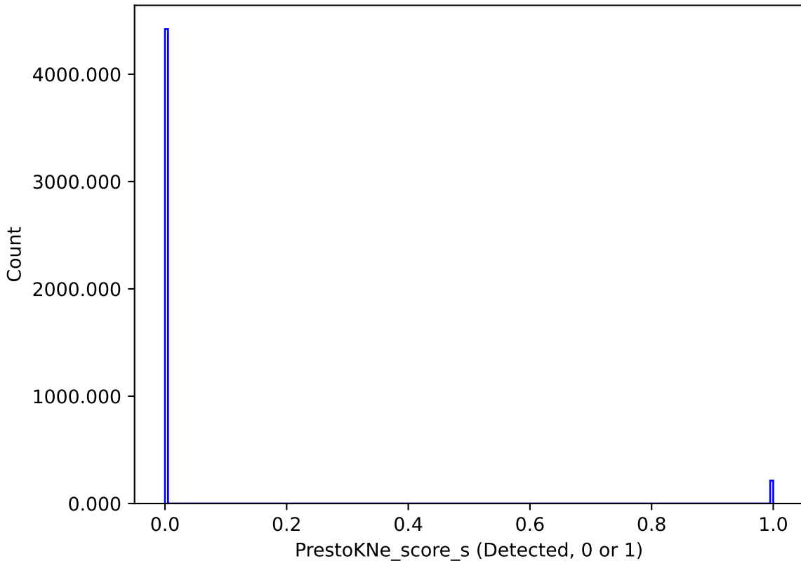
too_elab_r32_d3_ugrizy_v3.4_10yrs : PrestoKNe_score_s
