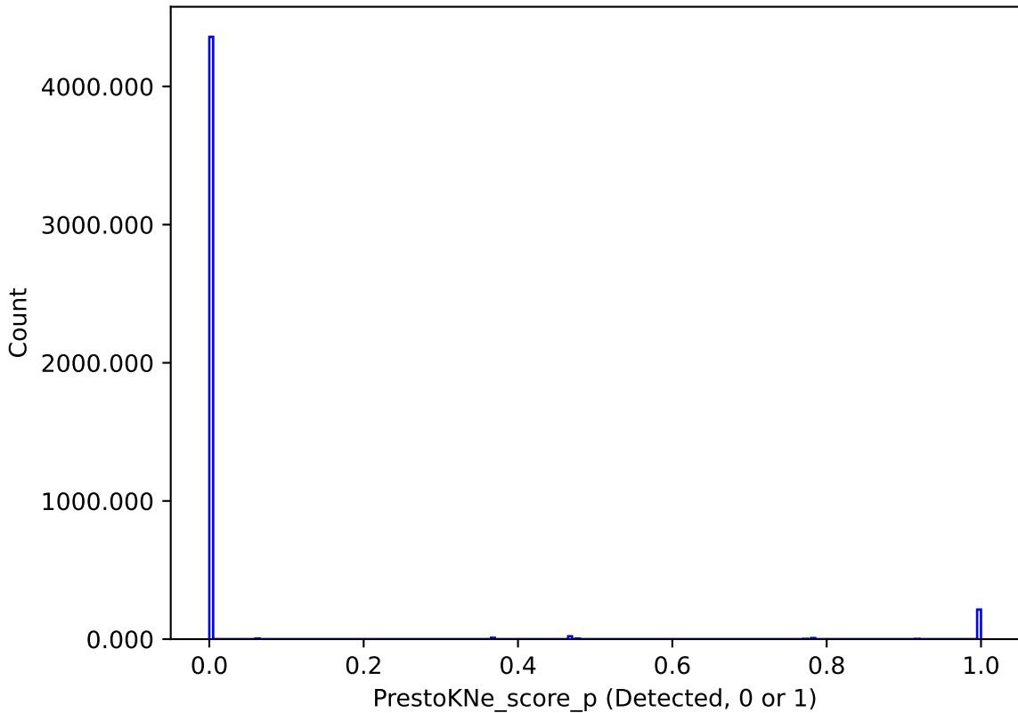
too_elab_r32_d3_ugrizy_v3.4_10yrs : PrestoKNe_score_p
