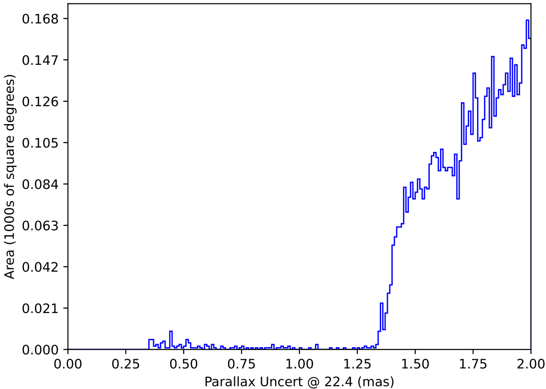
too_elab_r32_d3_ugrizy_v3.4_10yrs : Parallax Uncert @ 22.4
