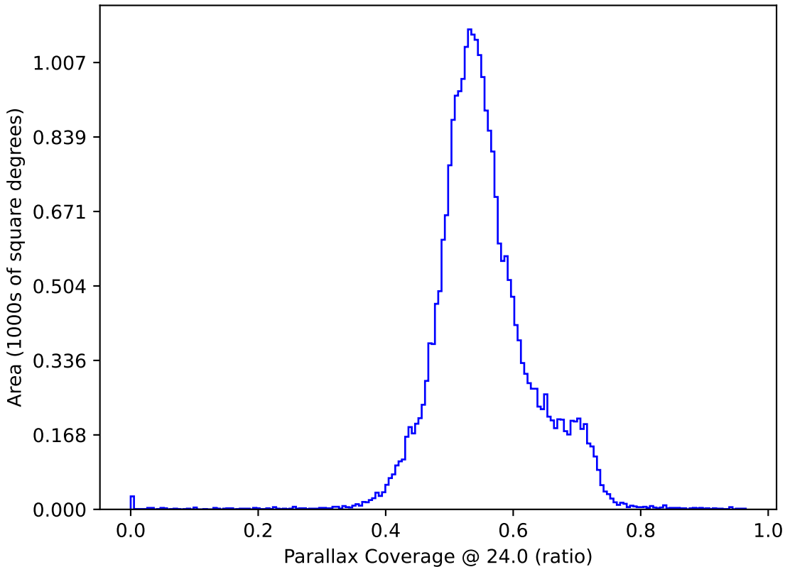
too_elab_r32_d3_ugrizy_v3.4_10yrs : Parallax Coverage @ 24.0
