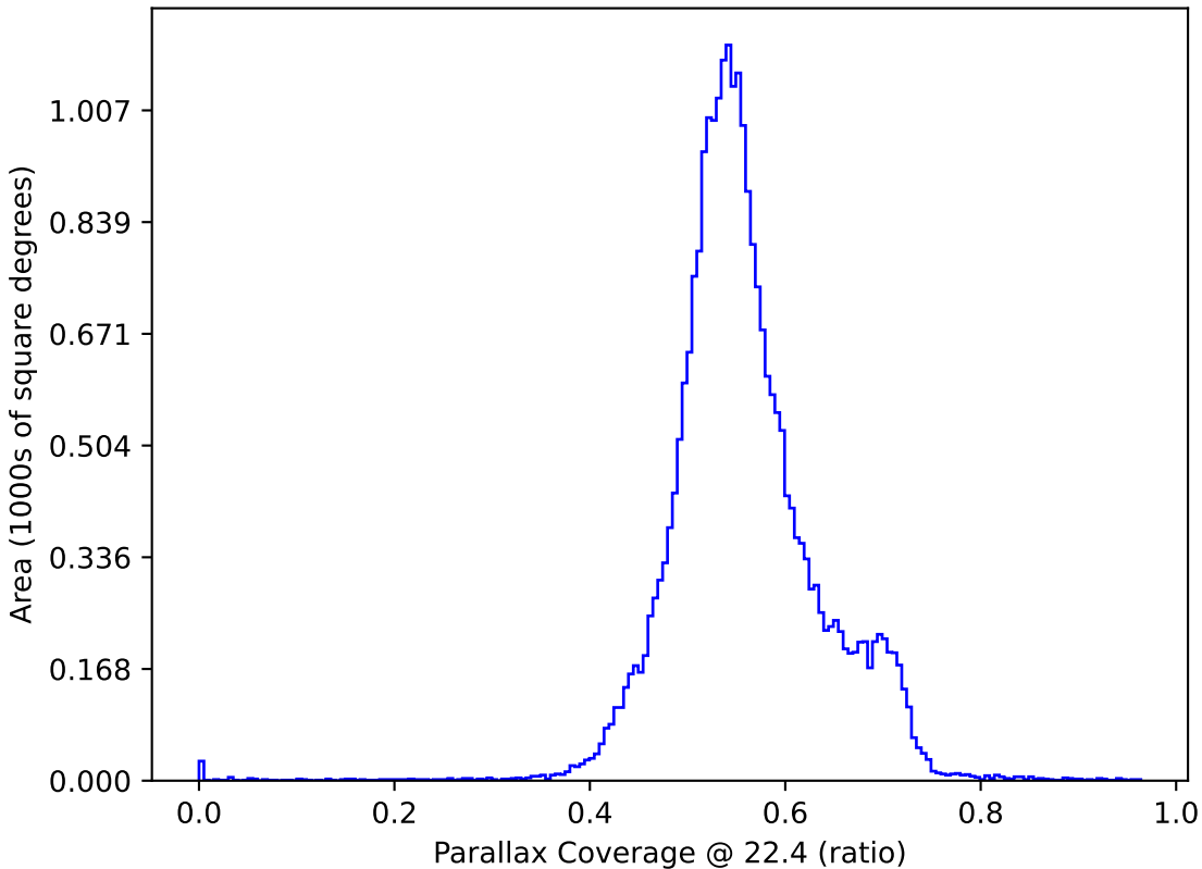
too_elab_r32_d3_ugrizy_v3.4_10yrs : Parallax Coverage @ 22.4
