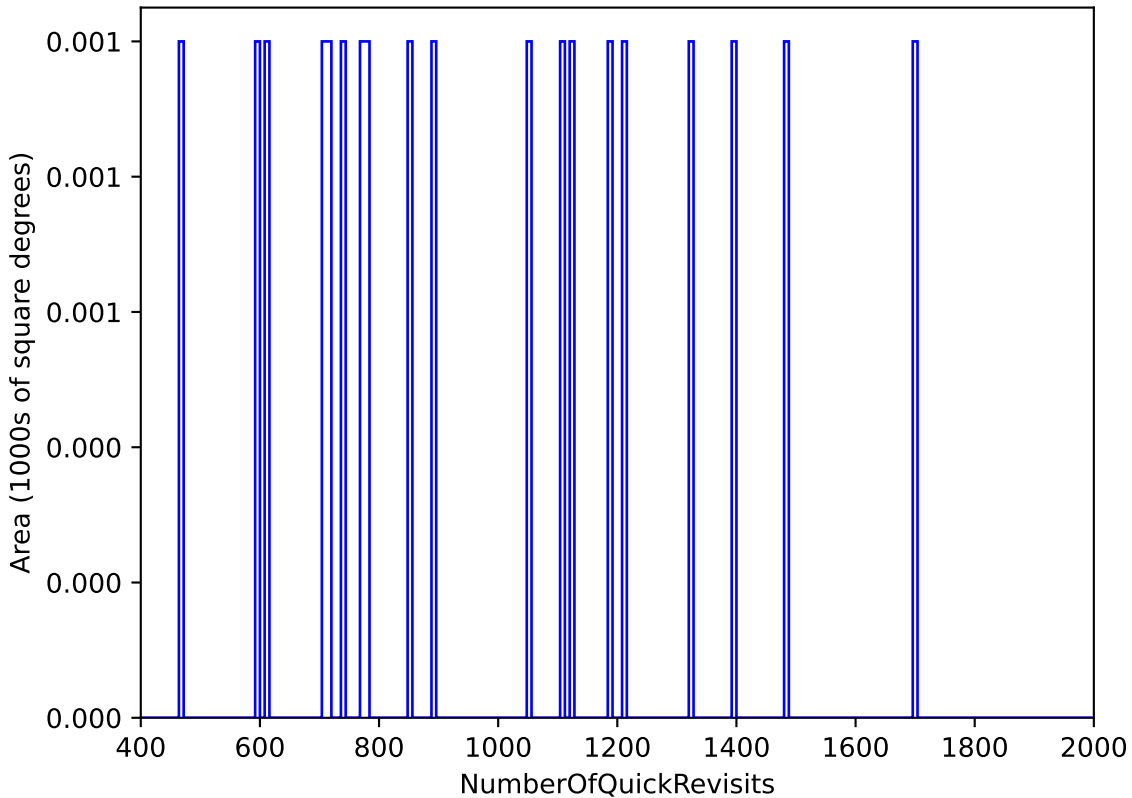
too_elab_r32_d3_ugrizy_v3.4_10yrs : NumberOfQuickRevisits
