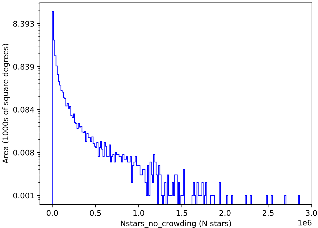
too_elab_r32_d3_ugrizy_v3.4_10yrs u: Nstars_no_crowding
