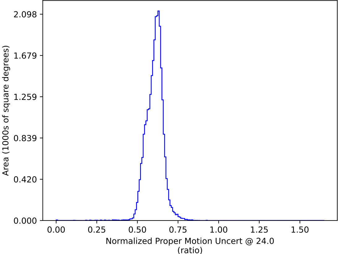
too_elab_r32_d3_ugrizy_v3.4_10yrs : Normalized Proper Motion Uncert @ 24.0
