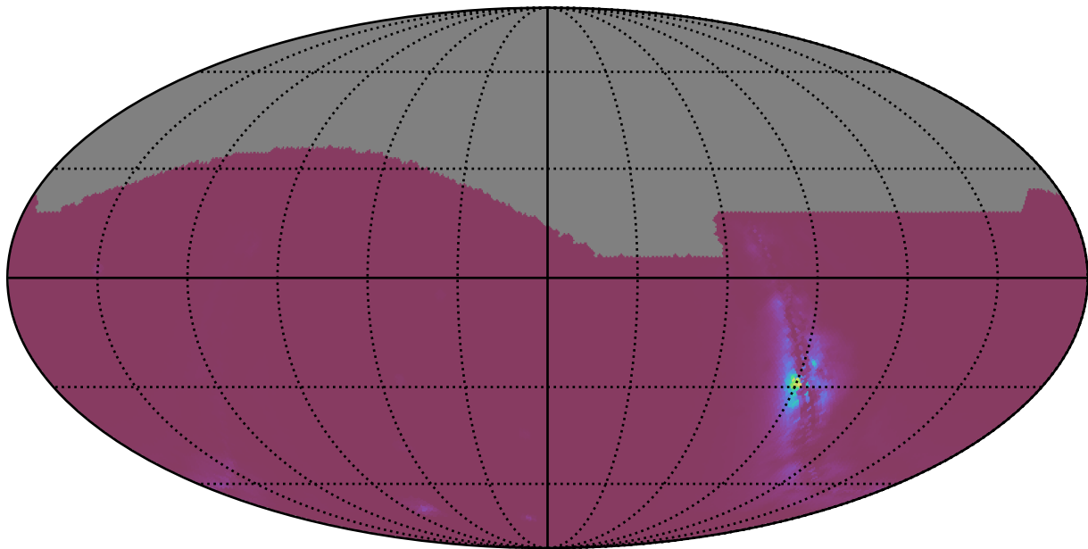
too_elab_r32_d3_ugrizy_v3.4_10yrs : NlcPoints
