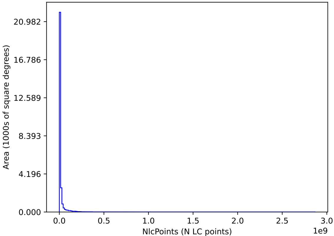
too_elab_r32_d3_ugrizy_v3.4_10yrs : NlcPoints
