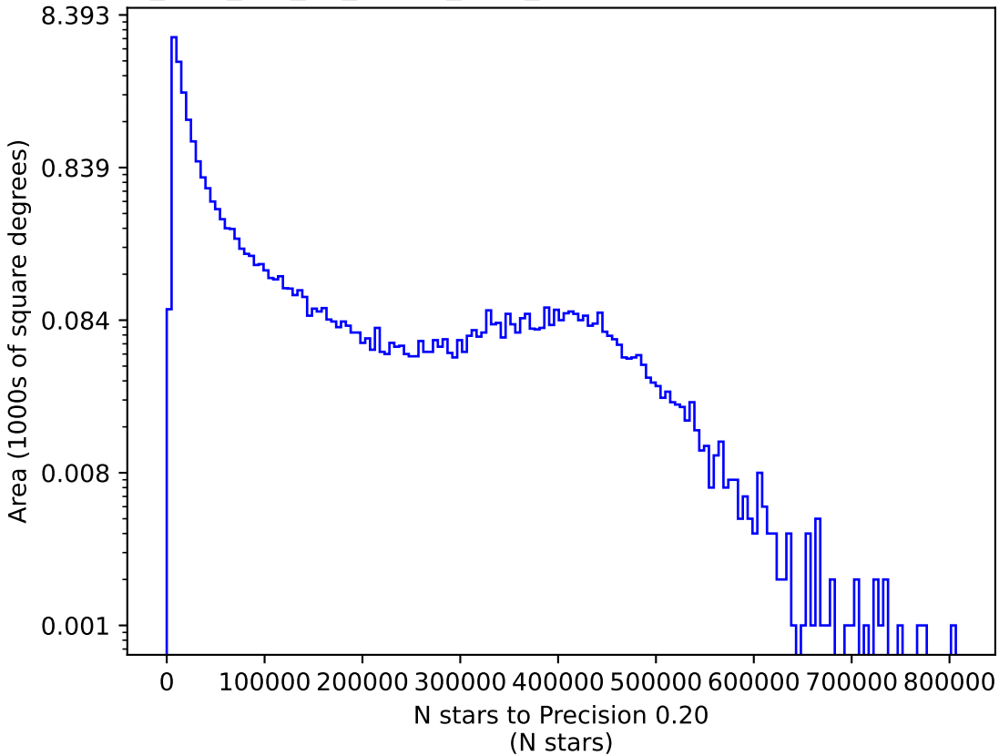
too_elab_r32_d3_ugrizy_v3.4_10yrs z: N stars to Precision 0.20
