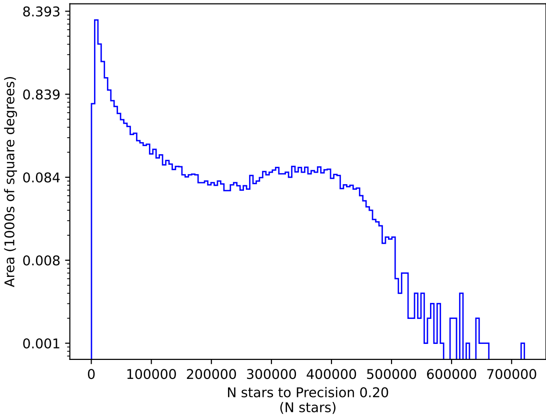
too_elab_r32_d3_ugrizy_v3.4_10yrs y: N stars to Precision 0.20
