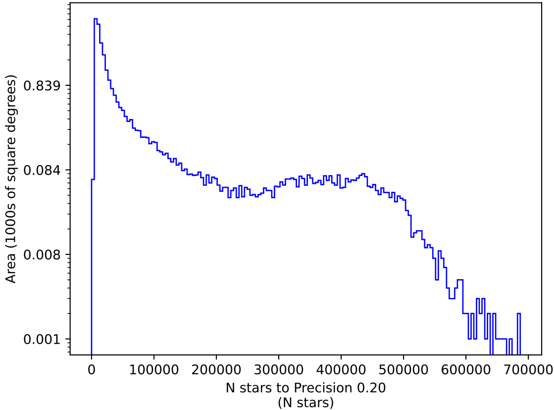
too_elab_r32_d3_ugrizy_v3.4_10yrs r: N stars to Precision 0.20
