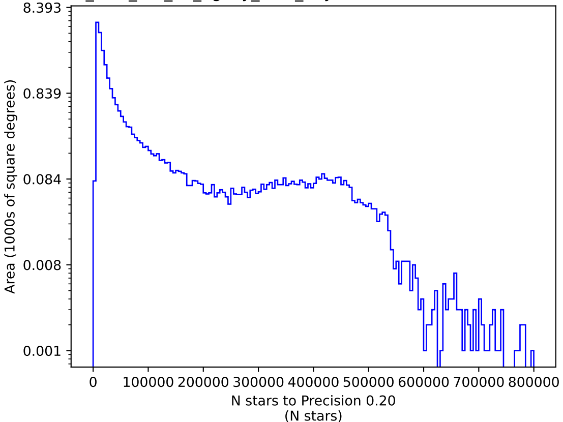
too_elab_r32_d3_ugrizy_v3.4_10yrs i: N stars to Precision 0.20
