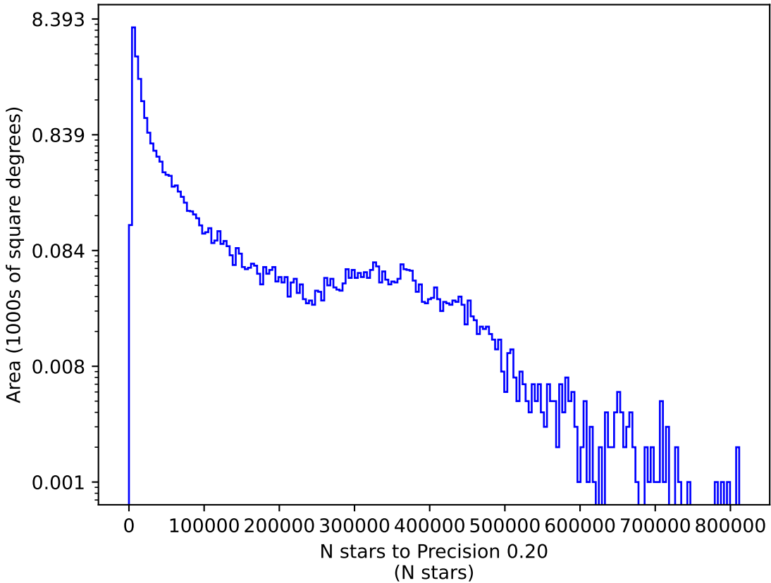
too_elab_r32_d3_ugrizy_v3.4_10yrs g: N stars to Precision 0.20
