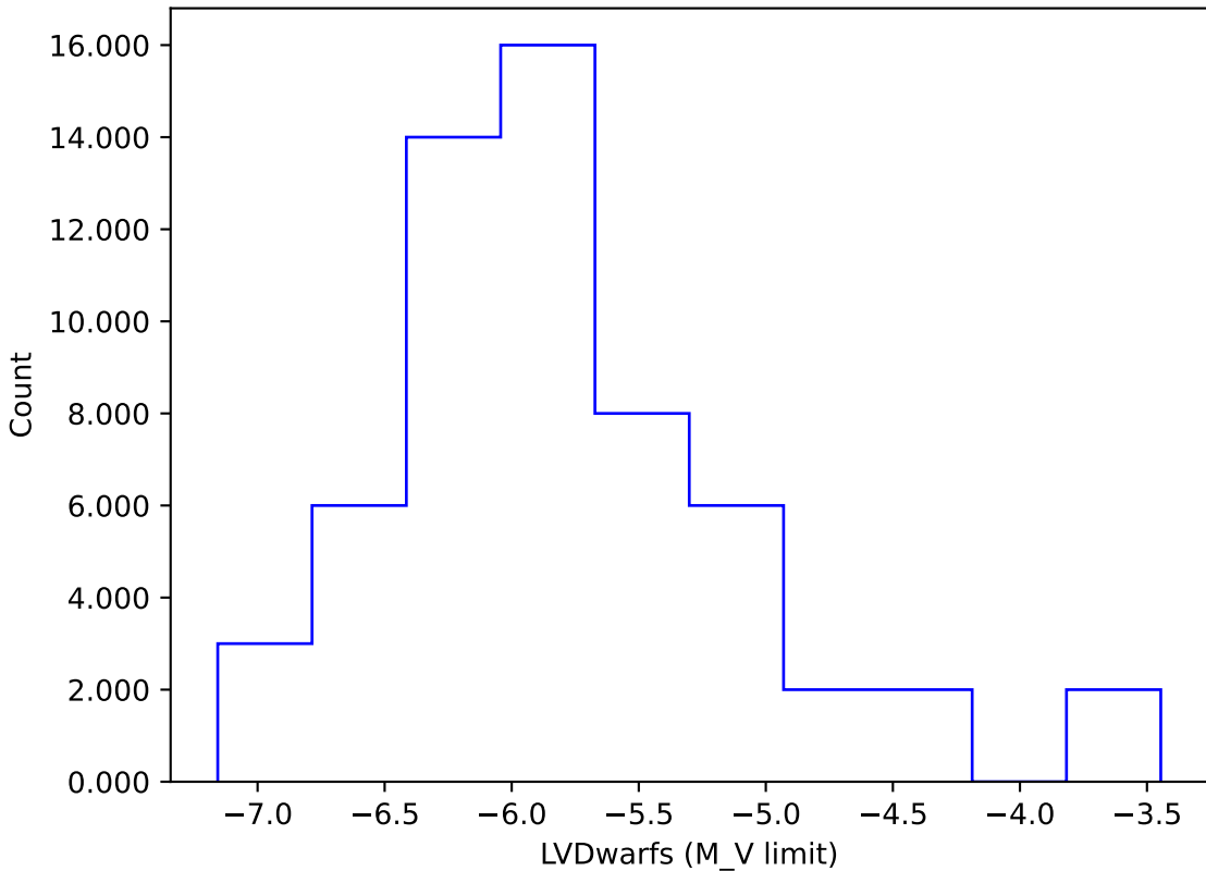
too_elab_r32_d3_ugrizy_v3.4_10yrs gi: LVDwarfs
