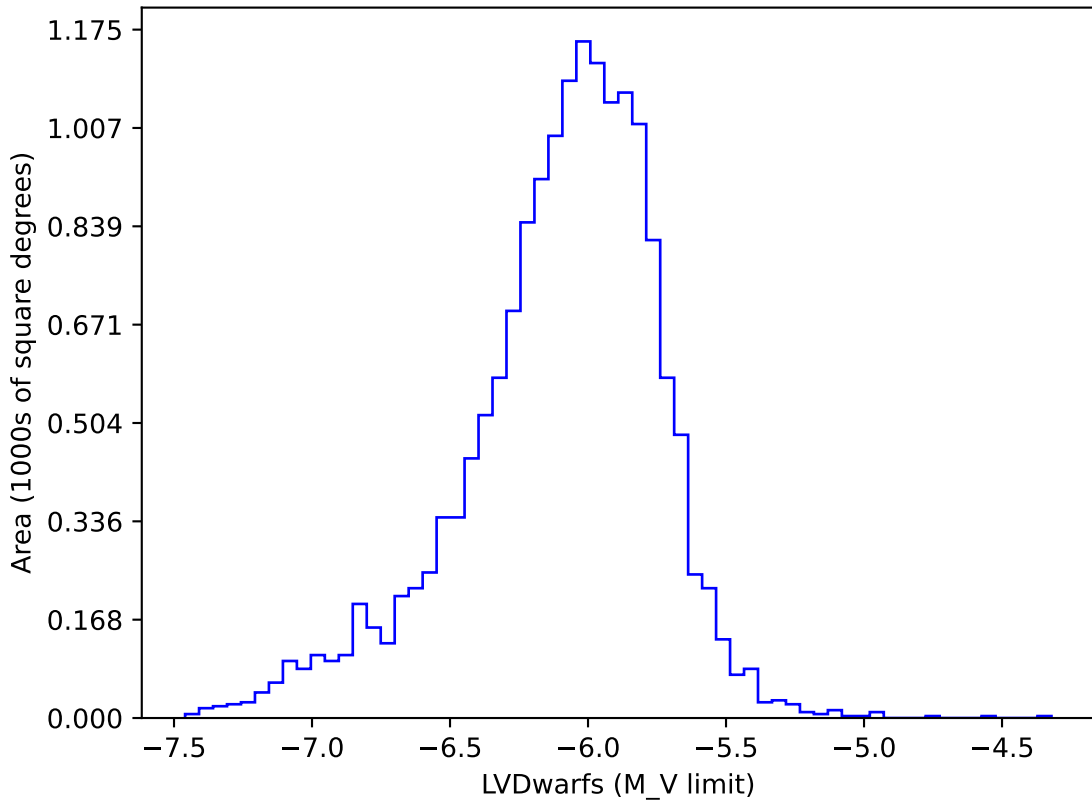
too_elab_r32_d3_ugrizy_v3.4_10yrs gi: LVDwarfs
