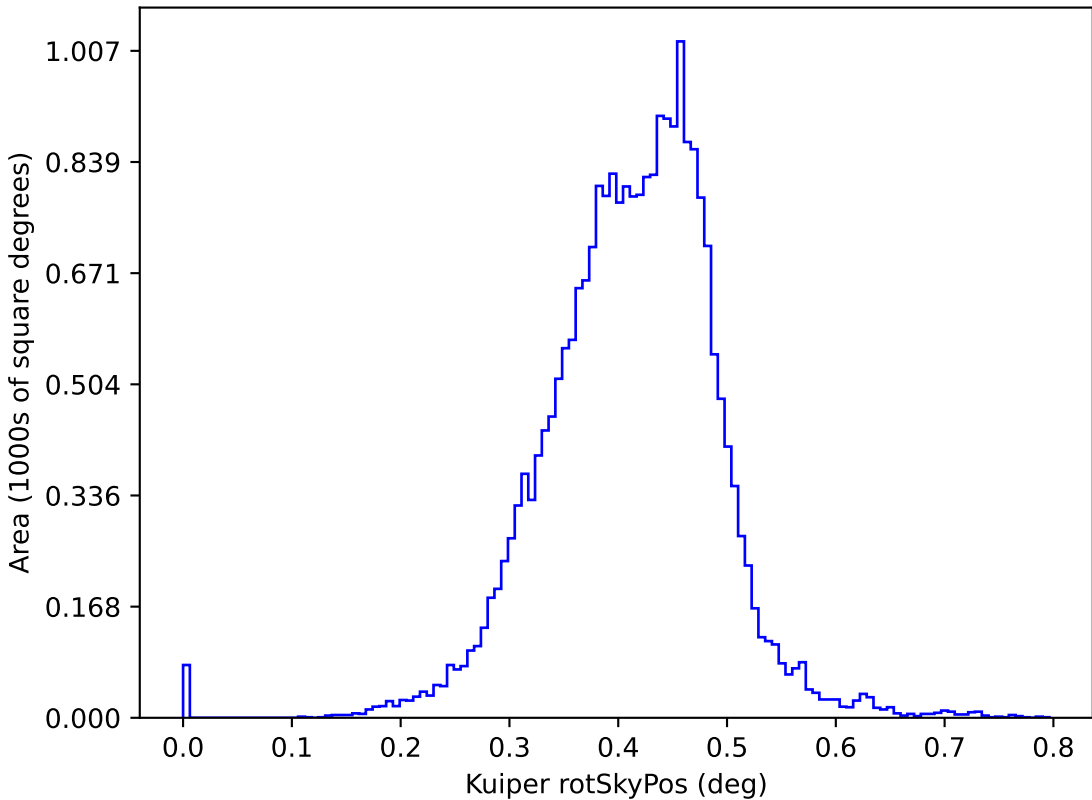
too_elab_r32_d3_ugrizy_v3.4_10yrs y: Kuiper rotSkyPos
