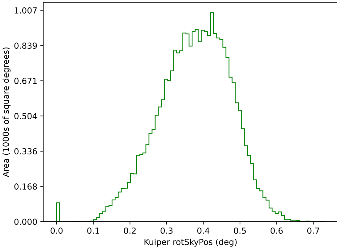
too_elab_r32_d3_ugrizy_v3.4_10yrs g: Kuiper rotSkyPos
