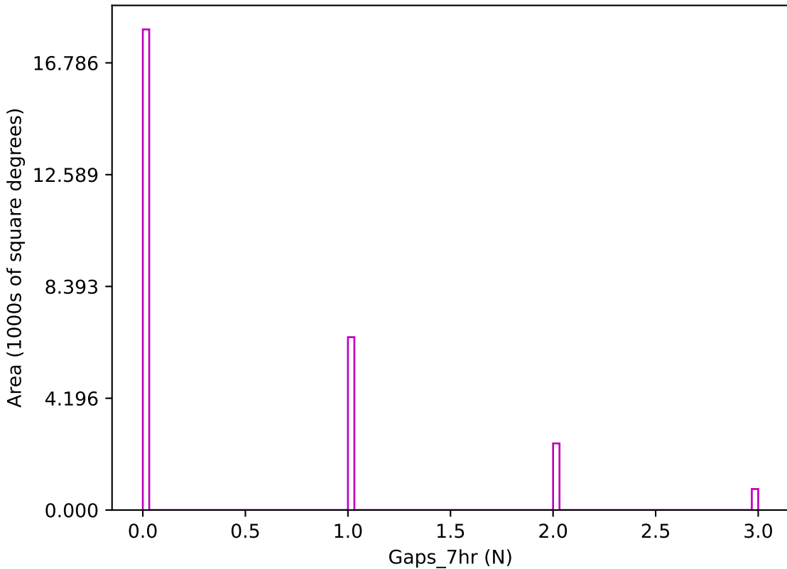
too_elab_r32_d3_ugrizy_v3.4_10yrs z band: Gaps_7hr
