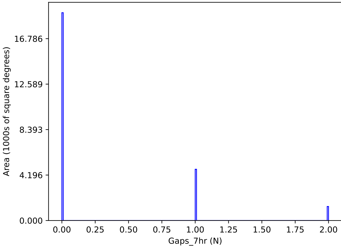
too_elab_r32_d3_ugrizy_v3.4_10yrs y band: Gaps_7hr
