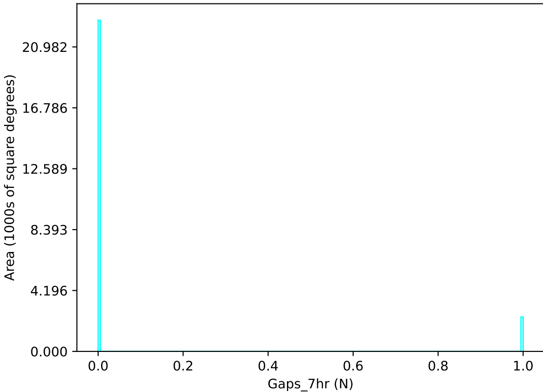
too_elab_r32_d3_ugrizy_v3.4_10yrs u band: Gaps_7hr
