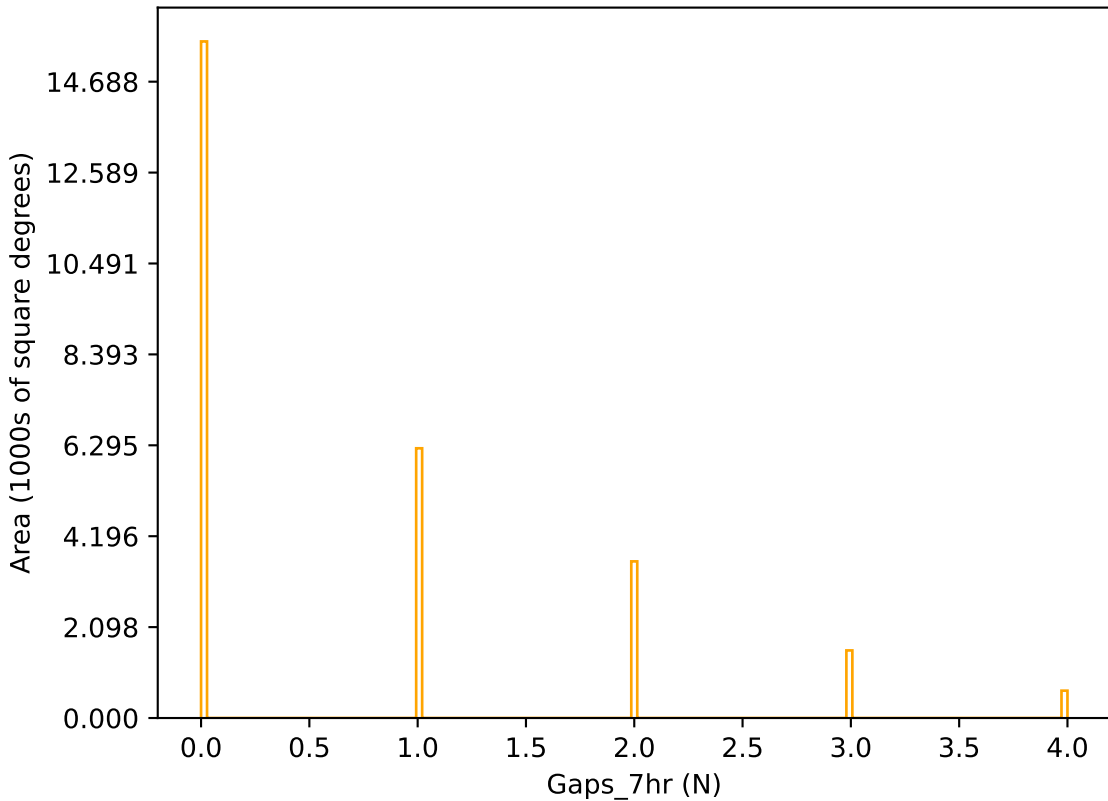
too_elab_r32_d3_ugrizy_v3.4_10yrs r band: Gaps_7hr
