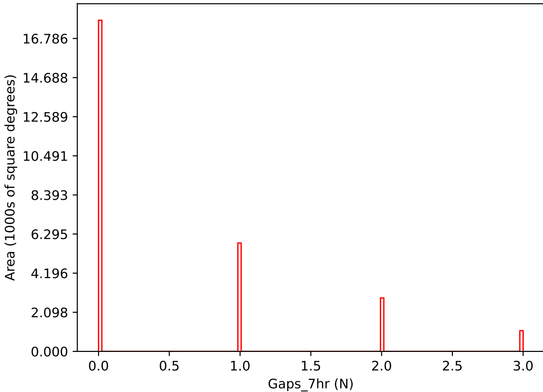
too_elab_r32_d3_ugrizy_v3.4_10yrs i band: Gaps_7hr
