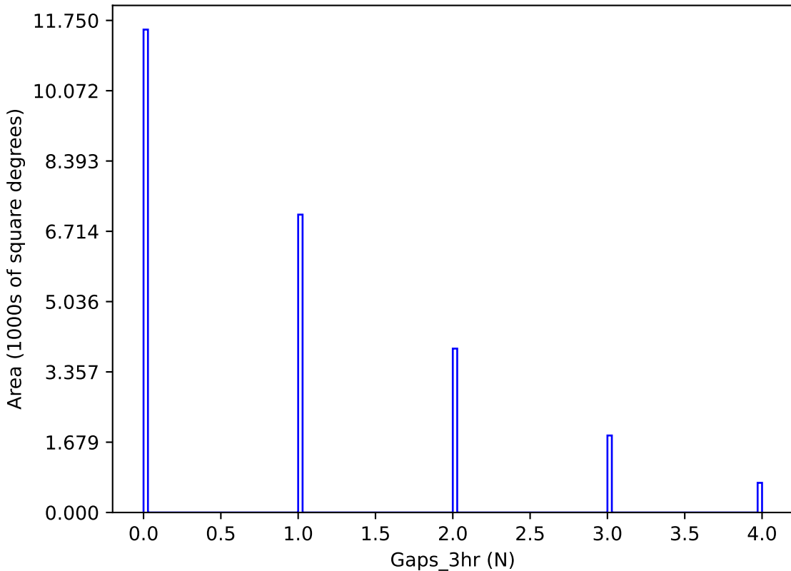
too_elab_r32_d3_ugrizy_v3.4_10yrs y band: Gaps_3hr
