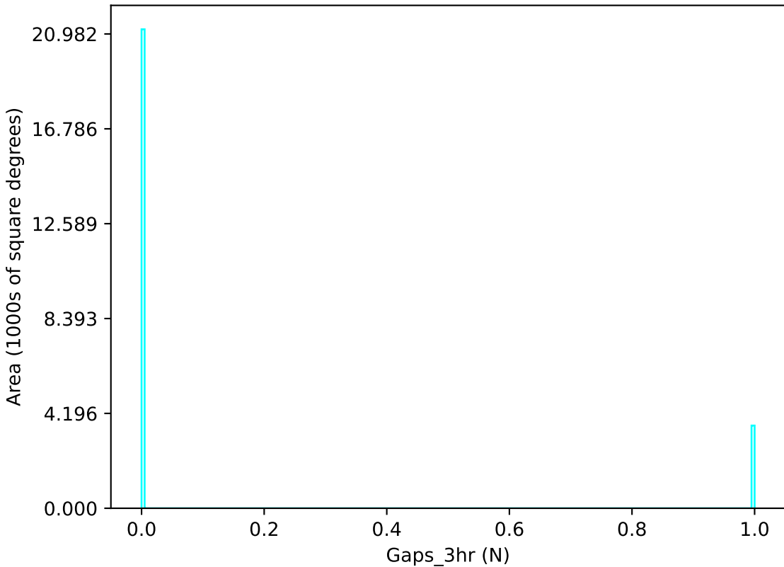
too_elab_r32_d3_ugrizy_v3.4_10yrs u band: Gaps_3hr
